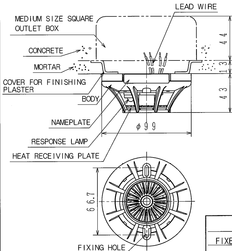
INSTALLATION WITH RECESS BOX
