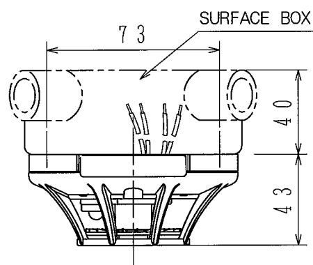
INSTALLATION WITH SURFACE BOX
